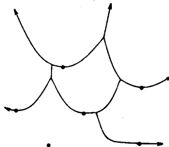
Fig. 2.3. V^* for points in Figure 2.1.
