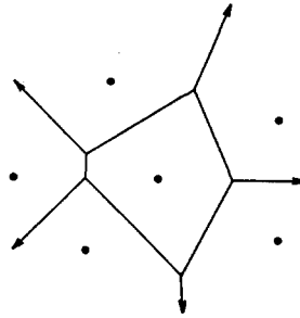
Fig. 2.1. Voronoi diagram V .
