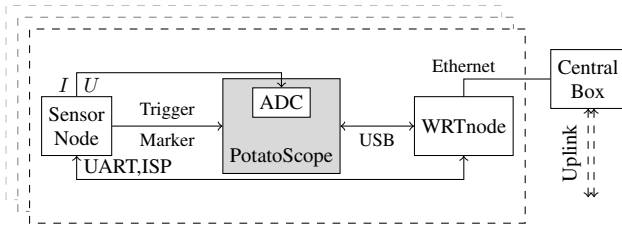
Fig. 1: PotatoNet architecture
