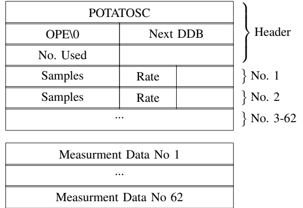
Fig. 3: Low Level Data Structure
