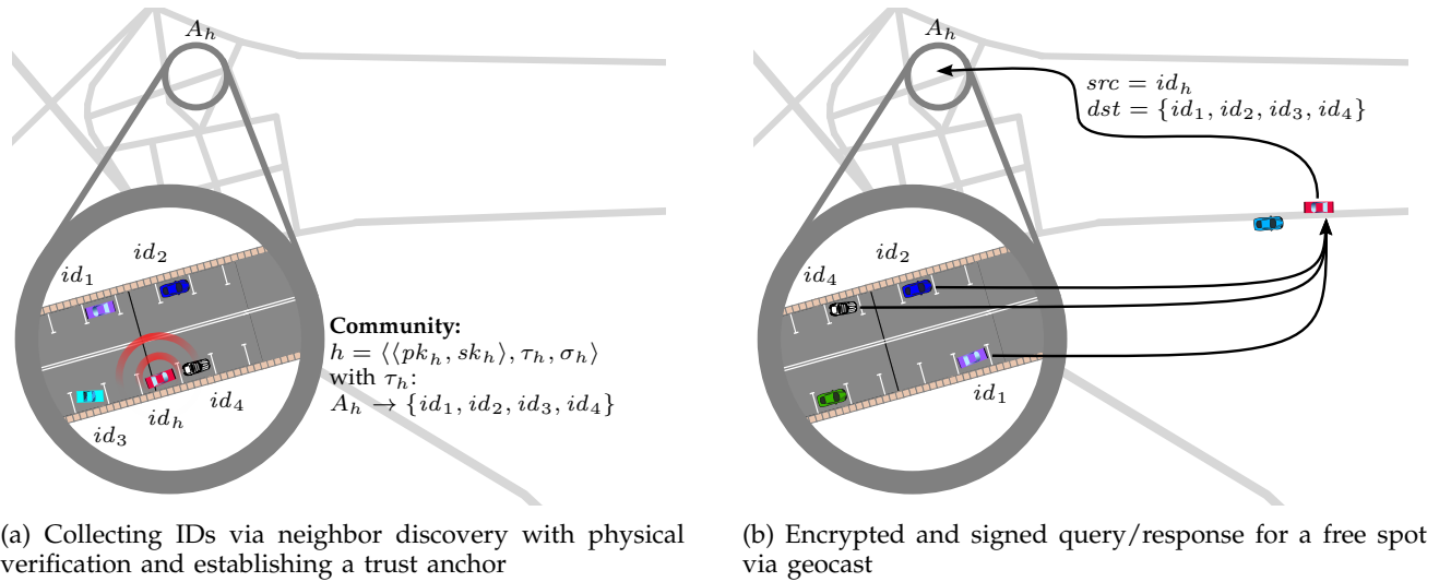
Figure 1: Creating and querying a Parking Community
